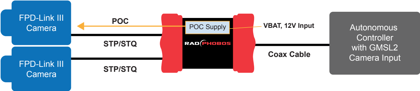
Power-over-coax from VBAT to camera / sensor.
